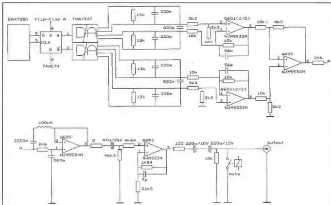
Marantz CD-10
